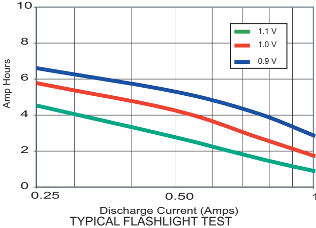
TYPICAL DISCHARGE CHARACTERISTICS AT 21°C (70°F)
